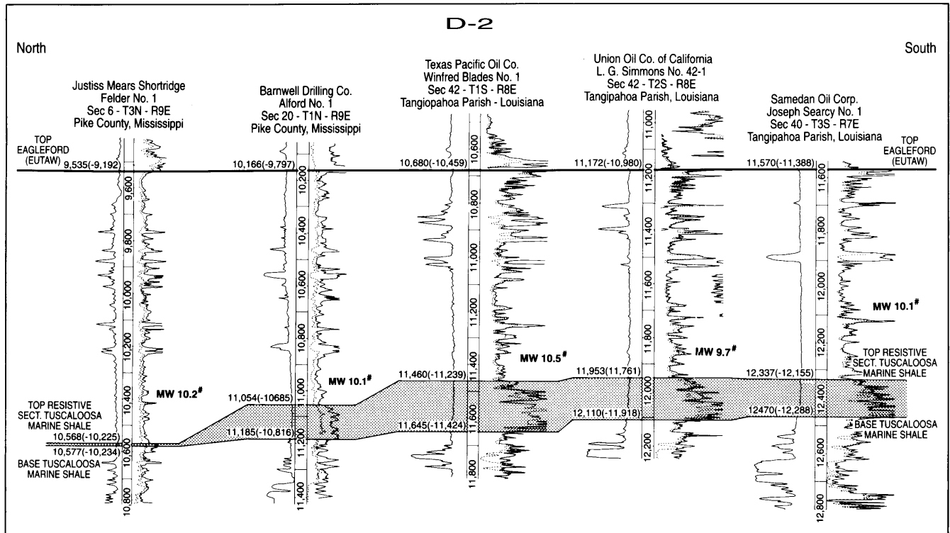
Figure 7. North-south dip section across the eastern part of the study area from Pike County, Mississippi to Tangipahoa Parish highlighting the resistive marine shale section. See figure 3 for the line of cross section (D-2). The Texas Pacific Oil Co., Winfred Blades No. 1 well, located in the center of this cross section is the only known well currently producing oil from the Tuscaloosa marine shale.
