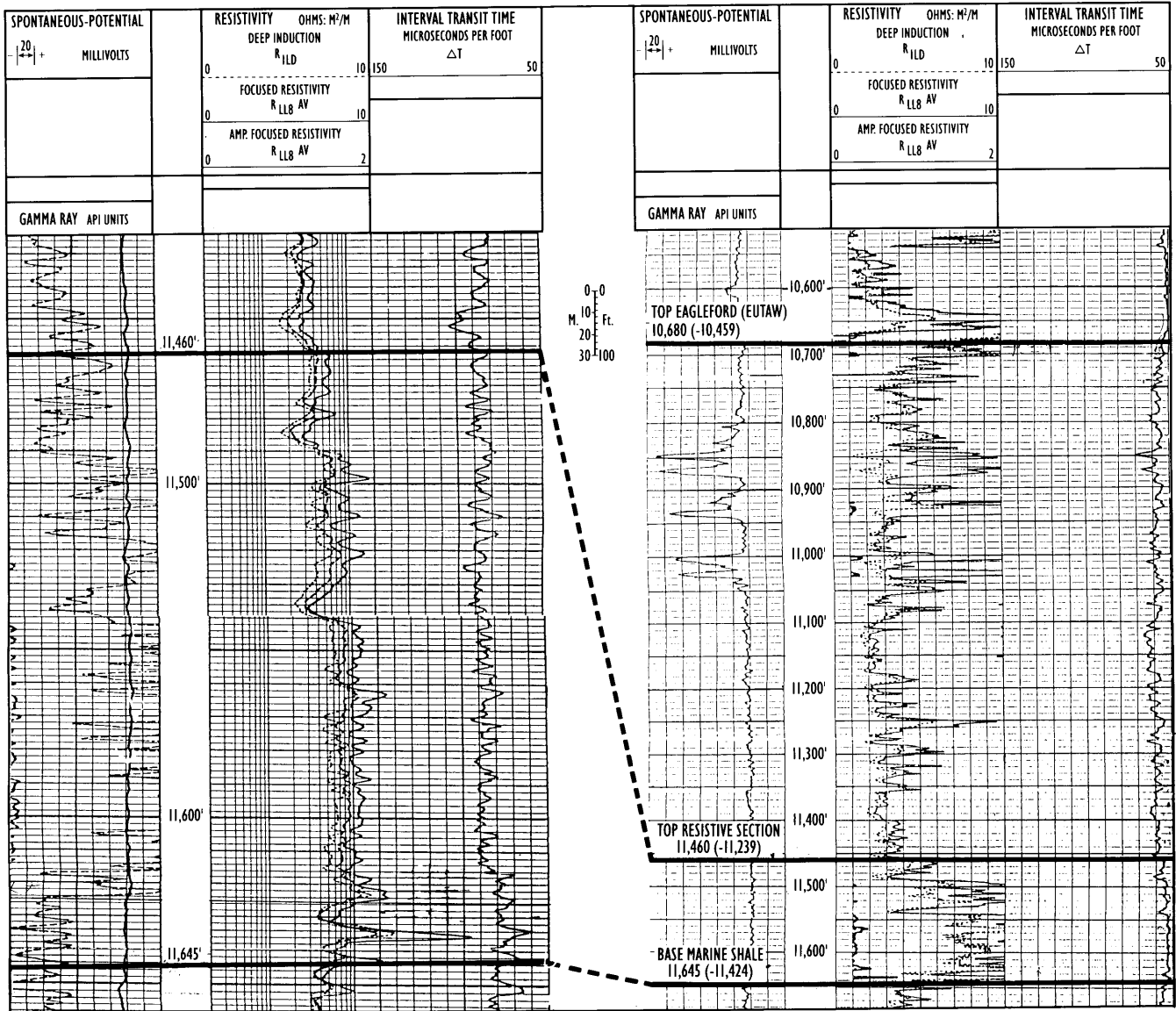
Figure 4. Type log of the marine shale section from the Texas Pacific Oil Company, #1 Winfred Blades, Tangipahoa Parish, Louisiana. The 1" log of the resistive section is shown on the right side and the 5" log is shown on the left side of the figure.
