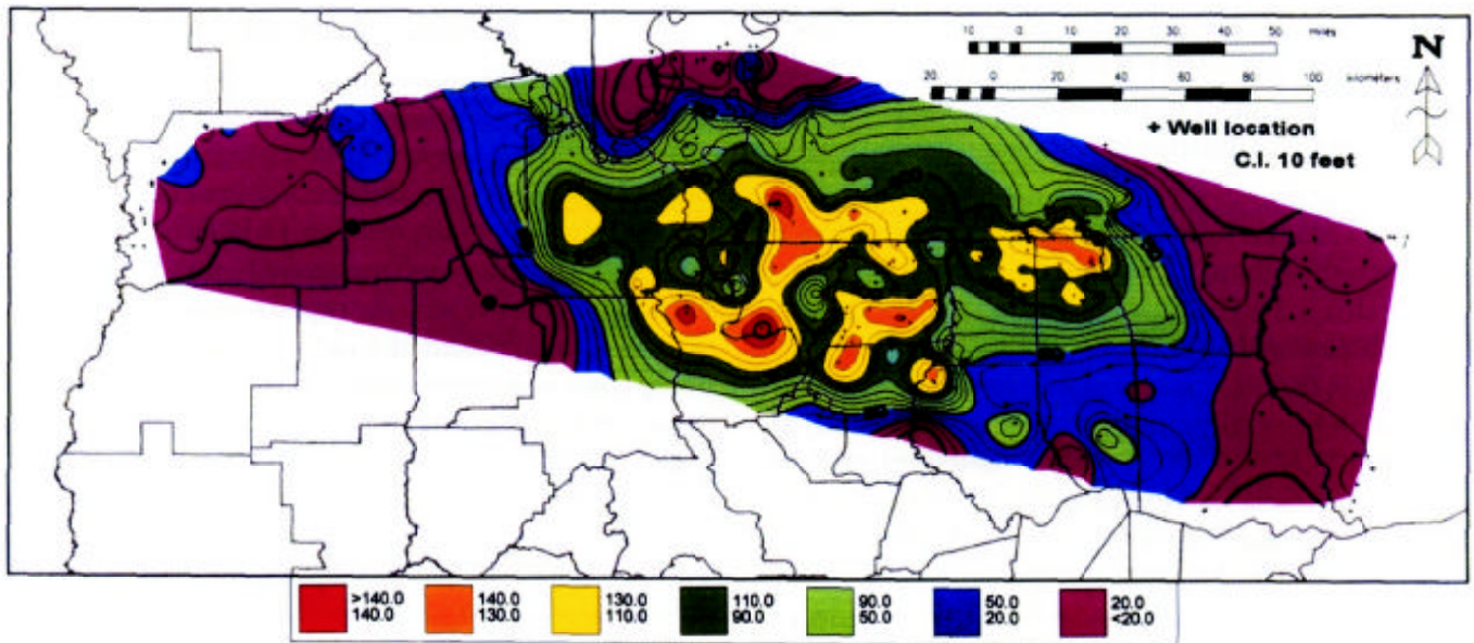
Figure 19. Net isopach map of the resistive Tuscaloosa marine shale section.
